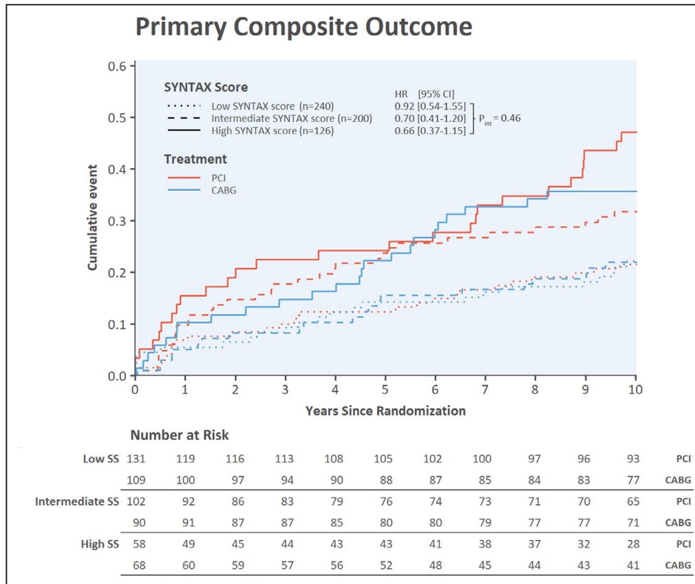
Figure 2. Ten-year event curves for primary end point of major adverse cardiac or cerebrovascular events according to the SYNTAX score categories and revascularization treatment.
