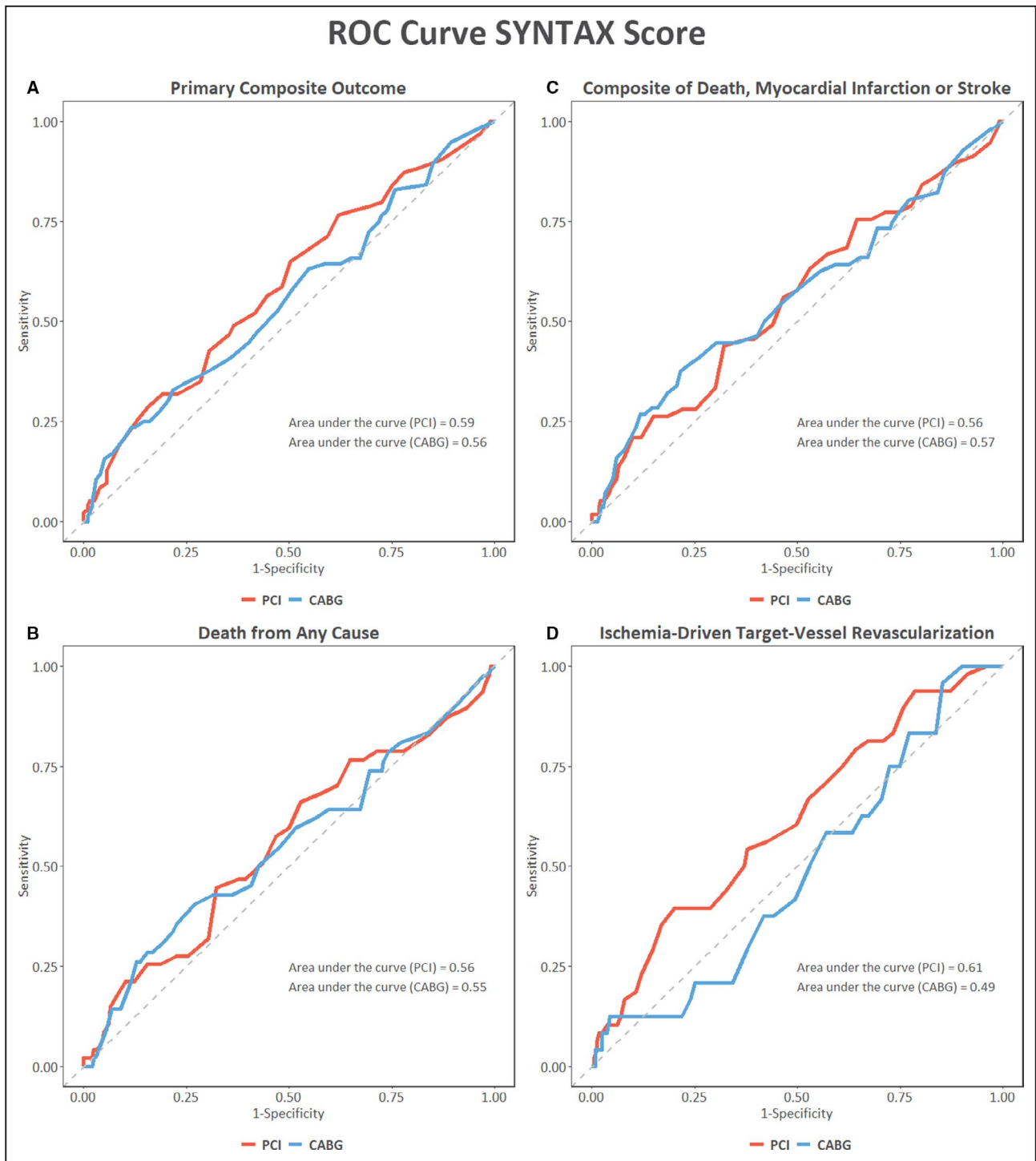
Figure 5. ROC curve for the discrimination capability of the SYNTAX score.
